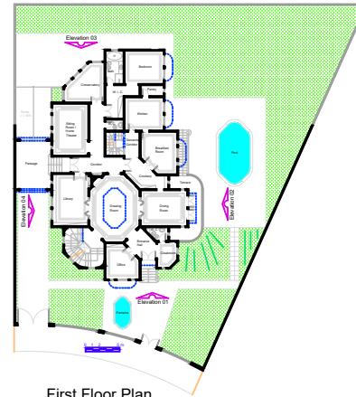
First Floor Plan A = 332,47 m 2
