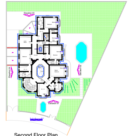
Second Floor Plan A = 289,04 m 2
